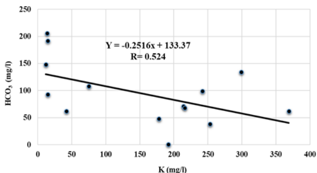
Figure 5 Linear regression model between the Bicarbonate (HCO 3 ) and the Potassium (K).
