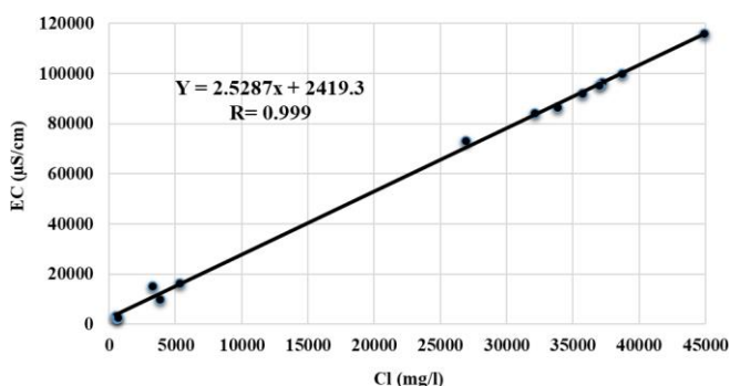
Figure 2 Linear regression model between the Chloride (Cl) and the Electrical Conductivity (EC).
