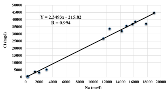
Figure 3 Linear regression model between the Sodium (Na) and the Chloride (Cl).
